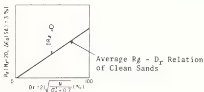
Fig. 27 Definition of DR_l
